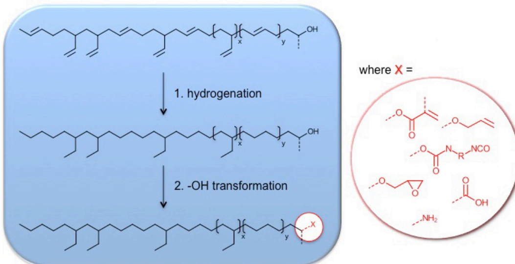
Figure 1: From polybutadiene monol to useful functional olefinic oligomers.
