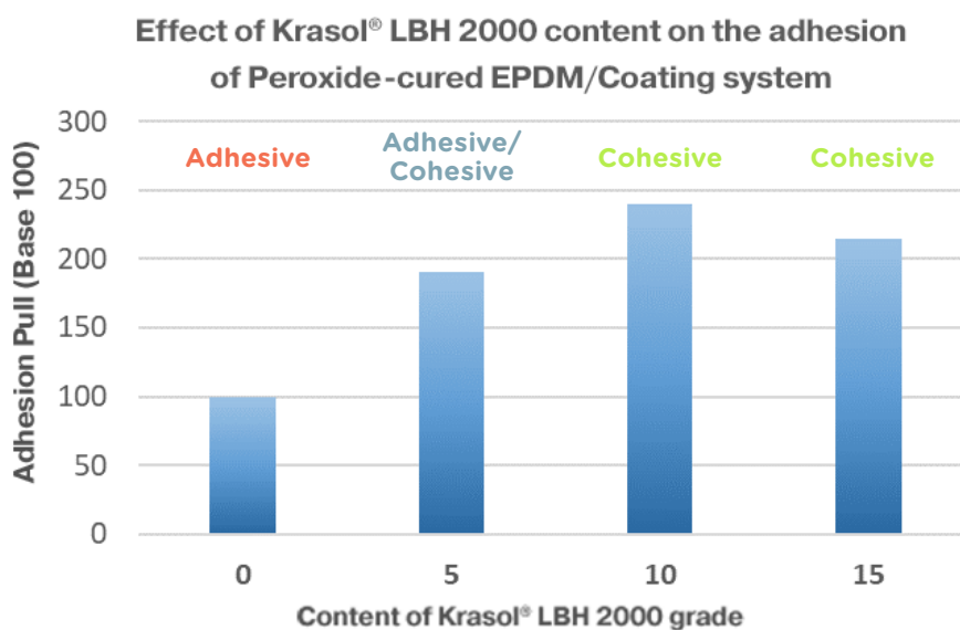
Figure 4: Results of T-peel tests with peroxide-cured EPDM compound and PU binder
